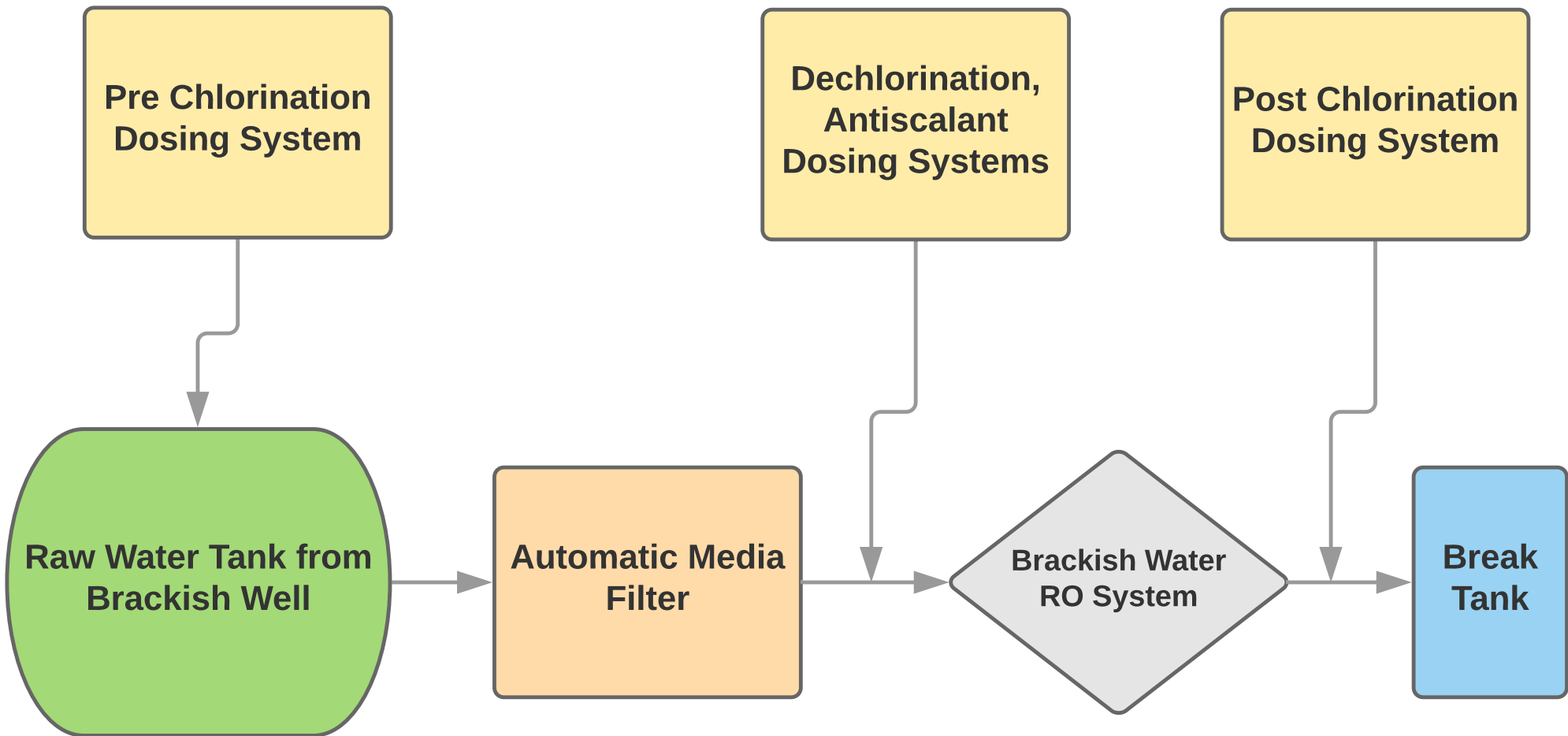
Industrial Reverse Osmosis System Flow Diagram
